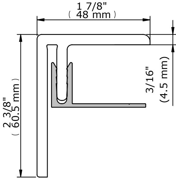
Tech-Wood® End profile Aluminum profile included
