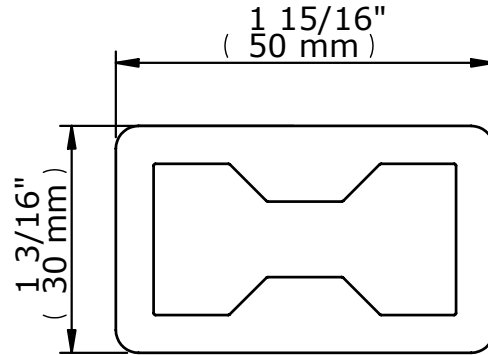
Tech-Wood® Joist
