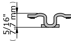
Tech-Wood® Stainless steel clip
