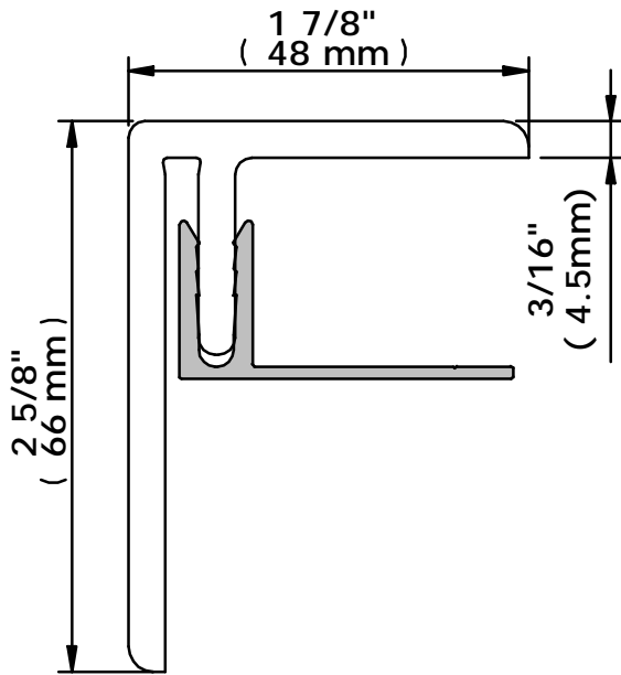
Tech-Wood® End profile Aluminum profile included
