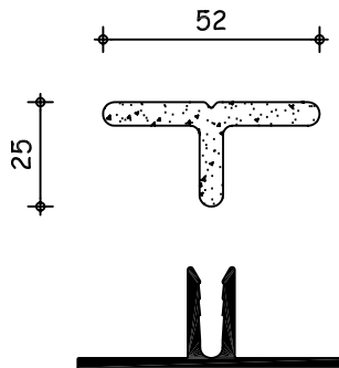
Tech-Wood® Expansion profile Aluminum profile included
