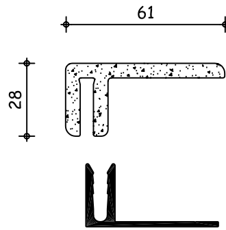
Tech-Wood® End profile Aluminum profile included
