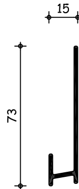
Tech-Wood® Starter profile
