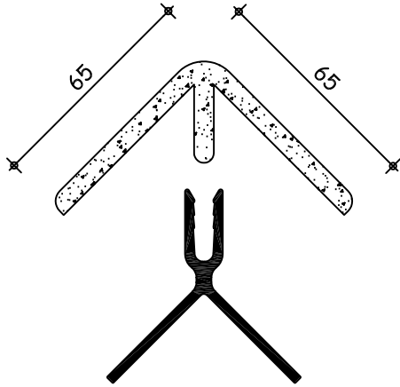
Tech-Wood® Corner profile Aluminum profile included
