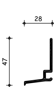
Tech-Wood® Starter profile for vertical installation of Channel-Siding
